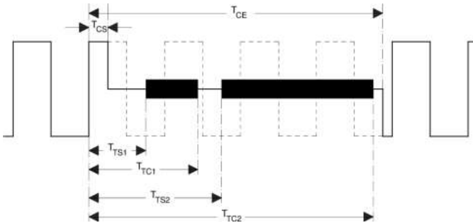
100 Figure 4: RailCom Timing
