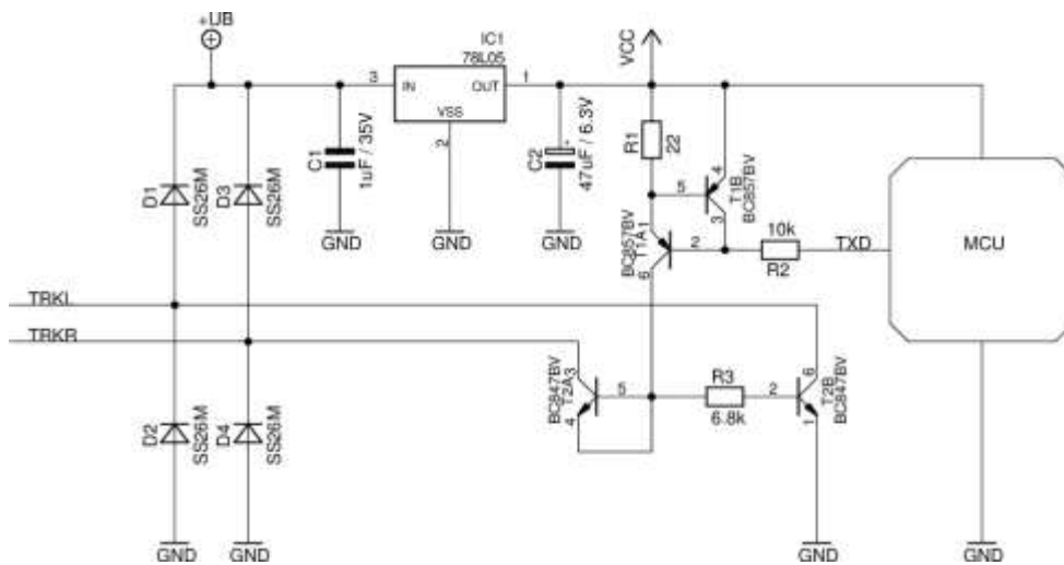
80 Figure 2: RailCom Decoder Hardware
