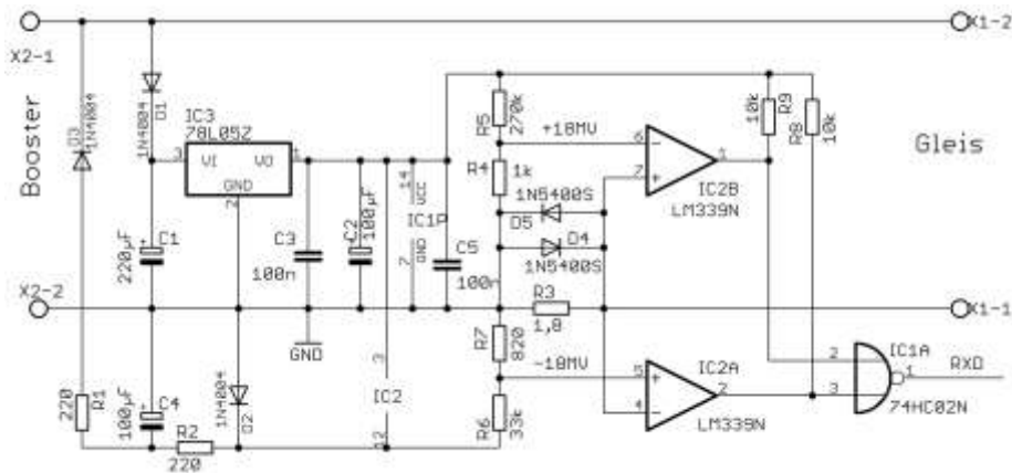
Figure 3: Example of a simple RailCom Detector Hardware
